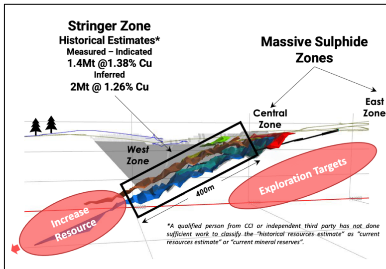
Figure 3: Chester Deposit Cross Section
