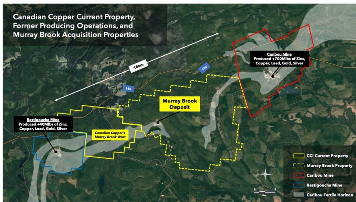
Figure A: Murray Brook Deposit Map
